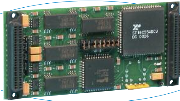
Large 64-byte FIFO buffers reduce the processing burden on the CPU to increase the overall system performance.
