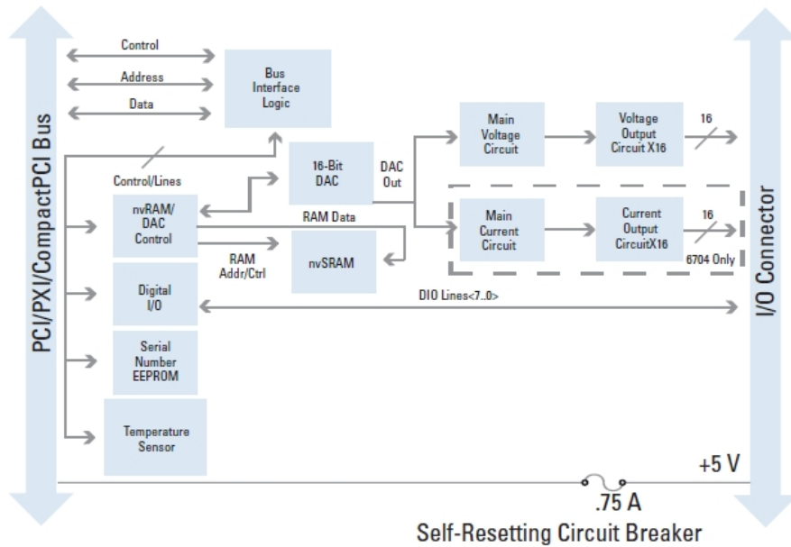
NI 670x Hardware Block Diagram
